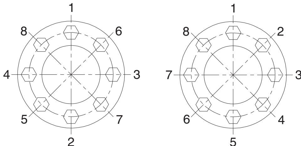
Figure 1 and 2 are examples of the typical tightening screw layouts. For exact number of screws refer to the appropriate RBL unit rating table.
